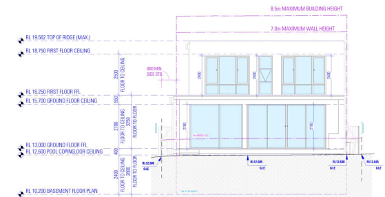
NORTH WEST ELEVATION 1
