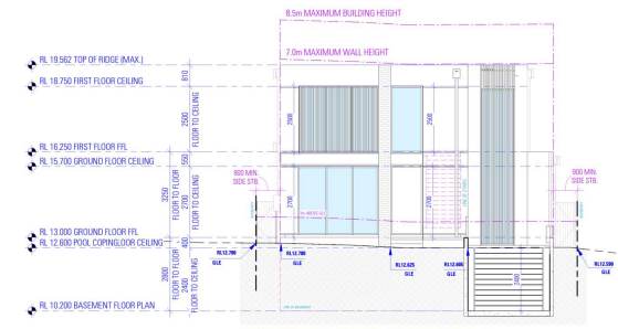
SOUTH EAST ELEVATION 1
